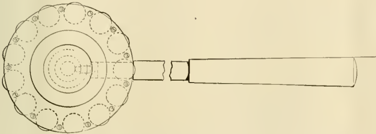
ROLLING AND EXPANDING DEVICE FOR TRIPLE VALVE BUSH.
